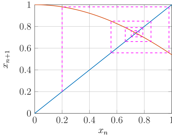
Figure 2.2: Starting from x_1 = 0.2 , the iteration in Example ?? maps x_n to x_{n+1} = \cos(x_n) . The points are also connected to the slope-1 line to show the path.
