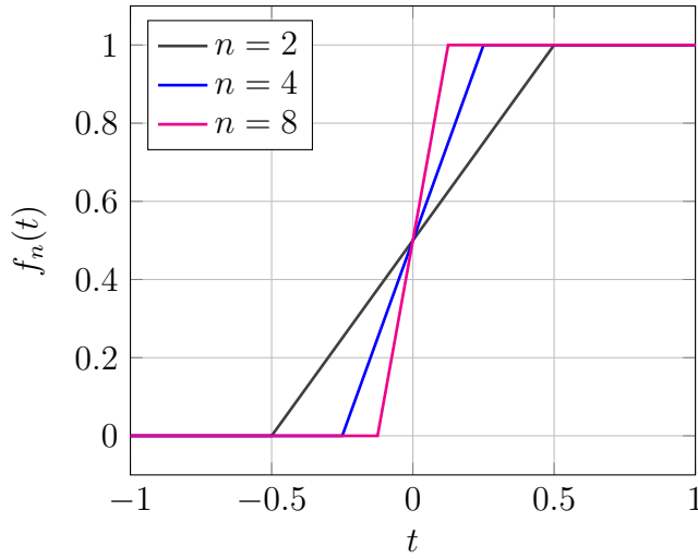
Figure 2.1: The sequence of continuous functions in Example ?? satisfies the Cauchy criterion. But, it does not converge to a continuous function in C[-1, 1] .
